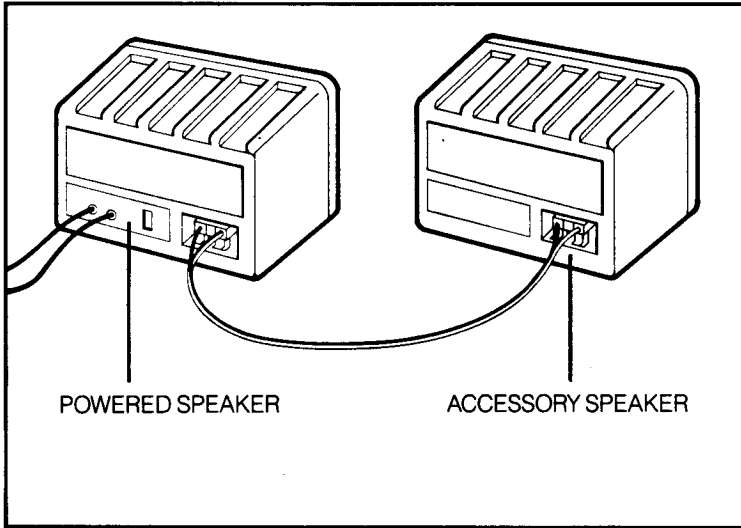
FIGURE 1 While the two enclosures look alike, they are different. The POWERED (LEFT) speaker also includes a stereo power amplifier.
